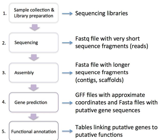
Fig. 1: The five steps involved in most genome projects: First, biological material is collected and the DNA and RNA are extracted and processed into sequencing libraries. Second, the libraries are sequenced, and the outputs from the sequencing machine (after much data filtering) are saved as a text file of inferred sequence "reads", typically in a FASTQ format text file. Third, based on sequence overlaps between reads, longer stretches of contiguous sequence ("contigs") are reconstructed and these contigs "strung together" into "scaffolds" representing chromosomal fragments. These contig and scaffold sequences are what is termed "the assembly". Fourth, in the gene feature annotation phase, automated programs and procedures are used to predict the approximate location of genes within the assembly (usually incorporating transcriptome data). Fifth, putative functions are assigned to the predicted genes based on homology to other species or prediction of conserved protein domains.
